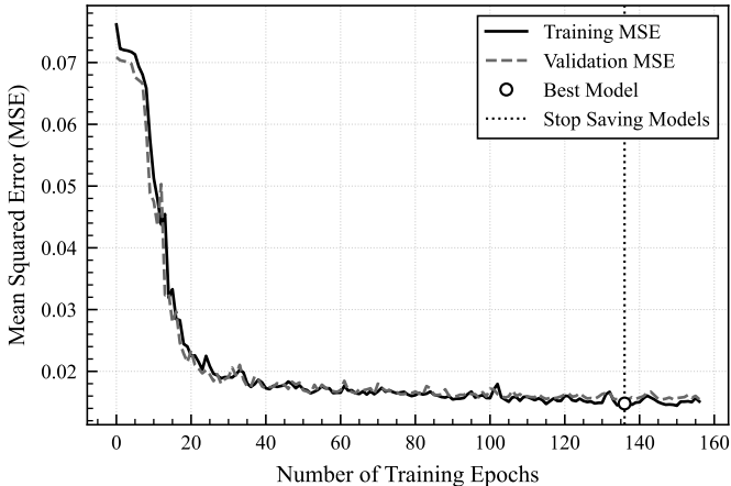
Learning Curve of GRU Model for SolarPlant-3 (Gyeongju)
